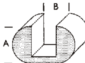
Randblei, rund / Lead came, U, round
